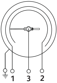
1 NO + 1 NC
