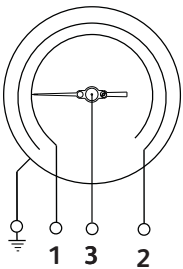
1 NC + 1 NO
