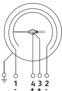
1 NO + 1 NC
