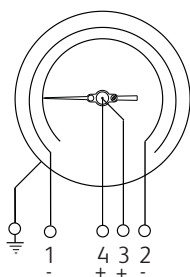
1 NO+ 1 NC
