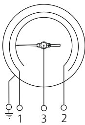
1 NO + 1 NC
