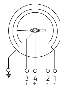
1 NC + 1 NC
